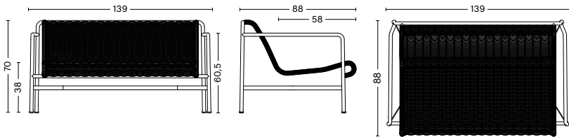
PALISSADE CORD LOUNGE SOFA Width 139 cm Depth 88 cm Height 70 cm Seat height 38 cm Seat depth 49 cm
