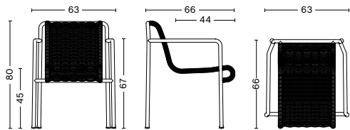
PALISSADE CORD DINING ARMCHAIR Width 63 cm Depth 66 cm Height 80 cm Seat height 45 cm Seat depth 44 cm
