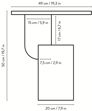
INSERT SIDE TABLE – FRONT VIEW
