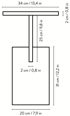
INSERT SIDE TABLE – SIDE VIEW
